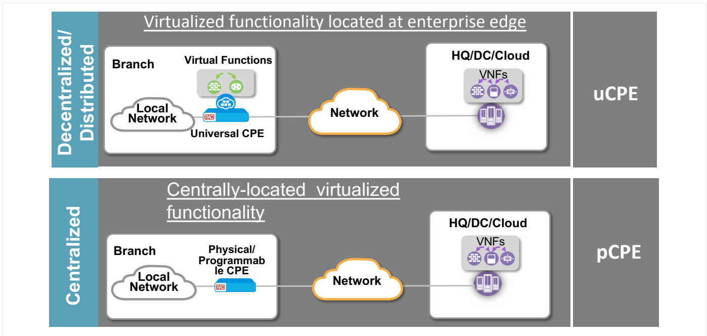
Figure 2. Comparison of centralized vs. decentralized approaches to virtualization.
